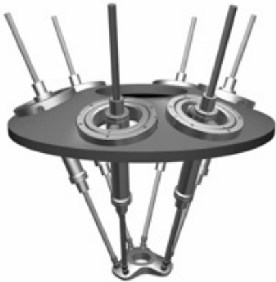
Hexapod Parallelkinematik
